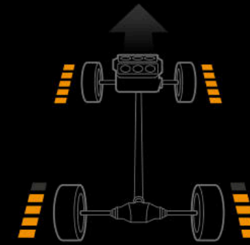
ACCELERATION
