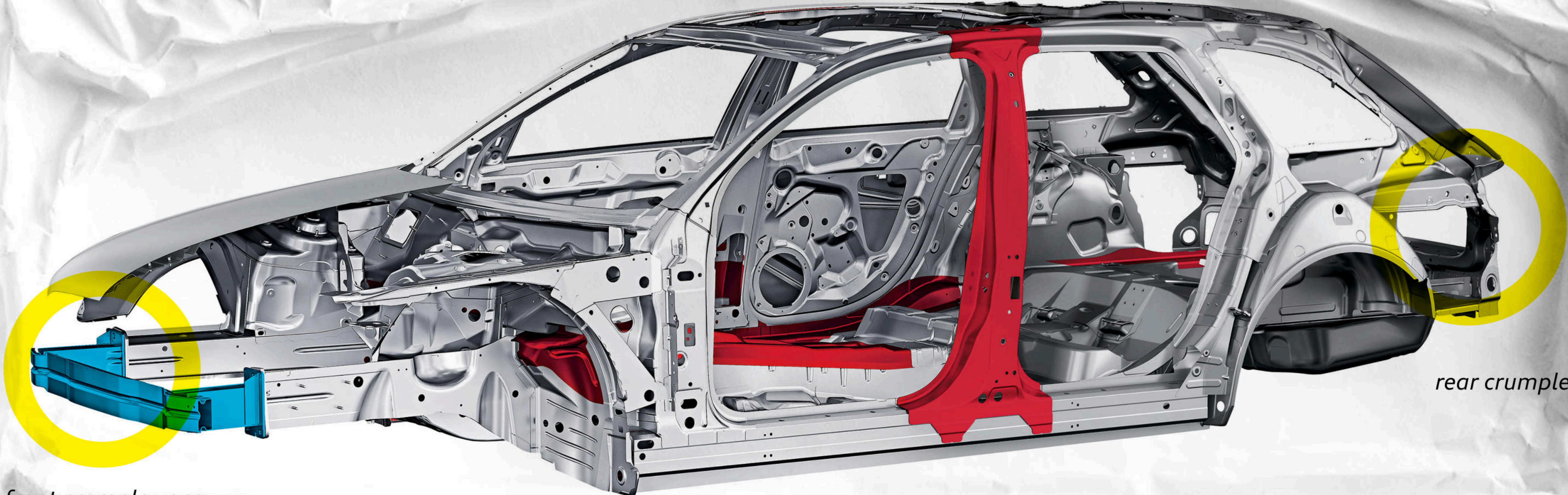
front crumple zone
