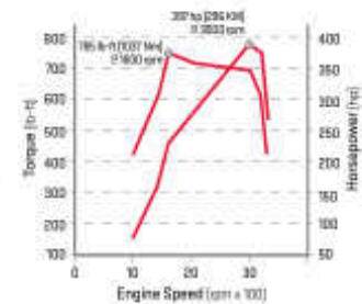
Duramax Diesel 6.6L V-8 Horsepower & Torque - SAE Certified
