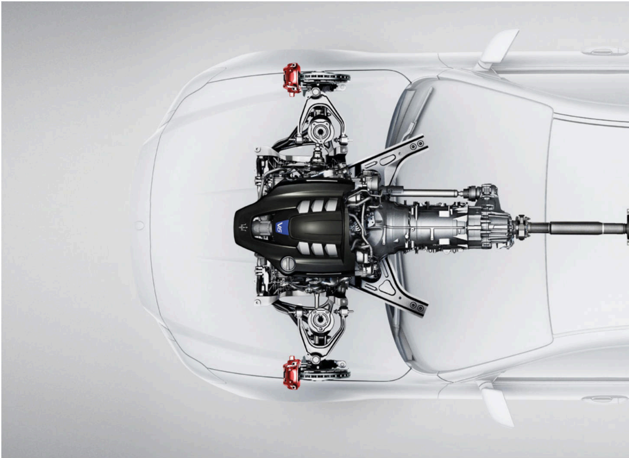
THE QUATTROPORTE S Q4 FEATURES AN ALL-WHEEL DRIVE SYSTEM THAT SUPPLIES TRACTION SEAMLESSLY ON DEMAND
