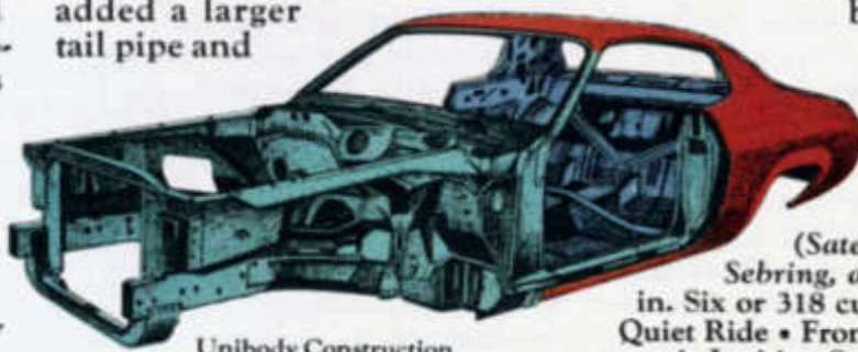
Unibody Construction
