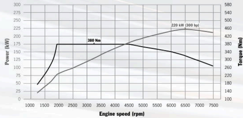
718 Boxster: 220 kW (300 hp) at 6,500 rpm, 380 Nm between 1,950 and 4,500 rpm
