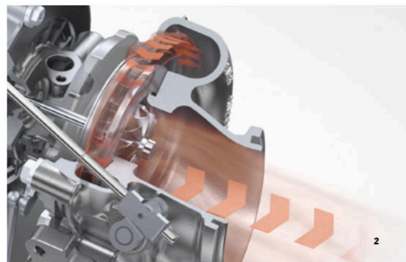
1 Turbocharger 2 Variable turbine geometry (VTG) of the S models
