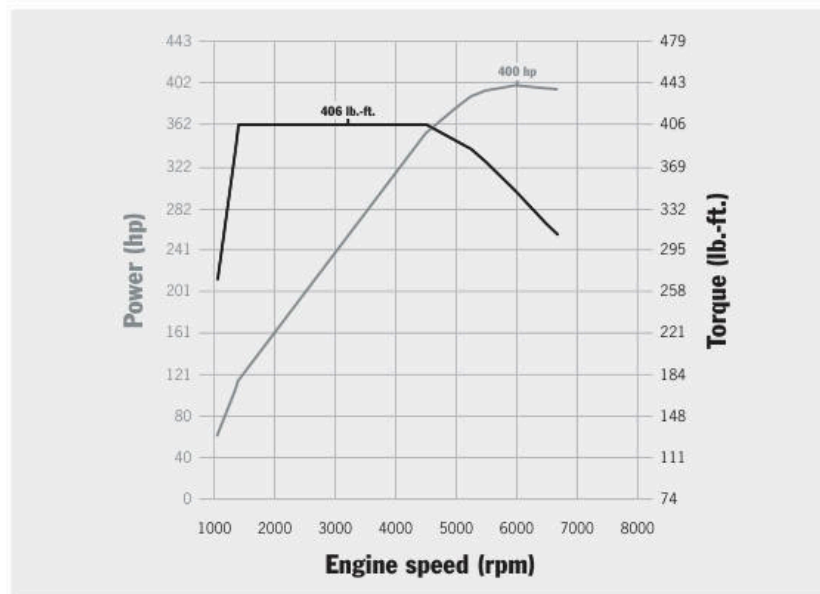
Macan Turbo: 406 lb.-ft. at 1350–4500 rpm, 400 horsepower at 6000 rpm
