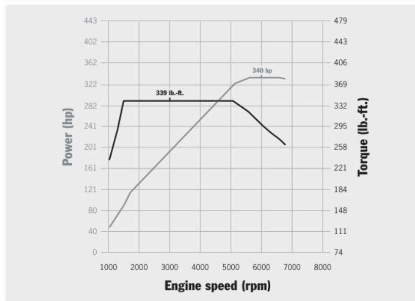
Macan S: 339 lb.-ft. at 1450–5000 rpm, 340 horsepower at 5500–6500 rpm
