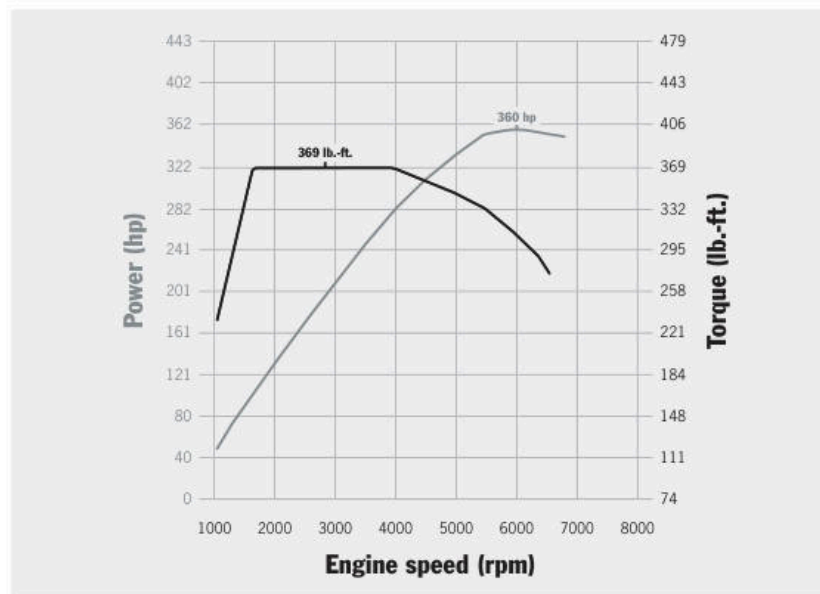
Macan GTS: 369 lb.-ft. at 1650–4000 rpm, 360 horsepower at 6000 rpm
