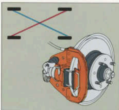
Independent brake circuit system (diagonally-divided). Disc brakes on all four wheels.
