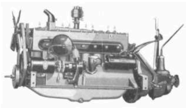
THE STUDEBAKER COMMANDER STRAIGHT EIGHT ENGINE Commander models are also offered with a six-cylinder engine.
