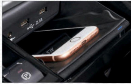
Wireless Charger. Conveniently charge your phone without the hassle of tangled wires. The Wireless Charger is a Qi Certified Device with Intelligent Charging Profiles, cell phone battery protection, temperature control technology and short circuit safe guards. Compatible with all Qi enabled devices and Samsung Fast Charge enabled devices. Anti-slip rubber insert safely holds your mobile device.
